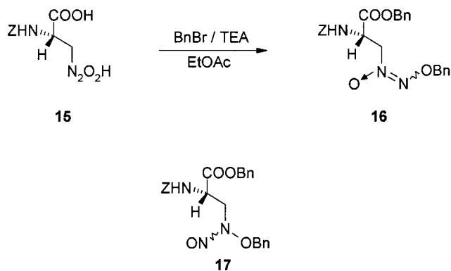
Scheme 8
