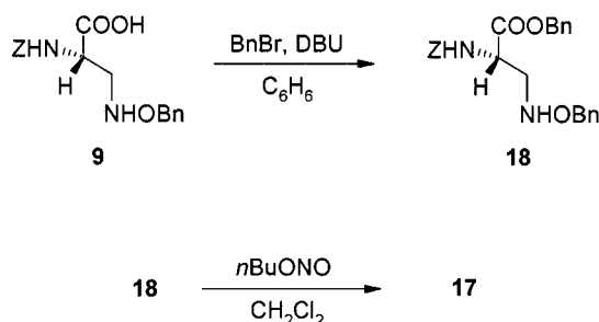
Scheme 9
