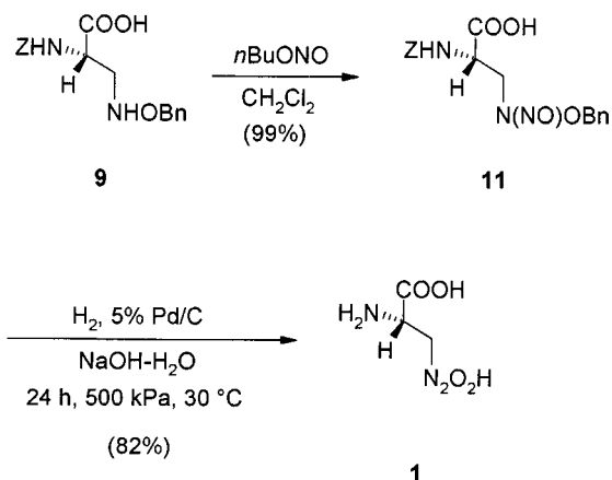
Scheme 6
